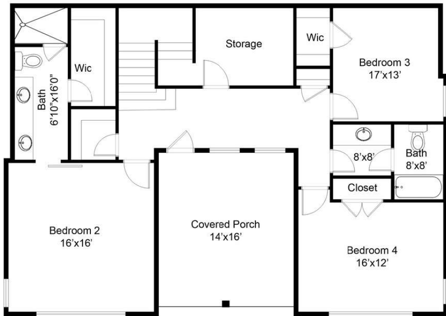
FOUNDATION FLOOR PLAN
