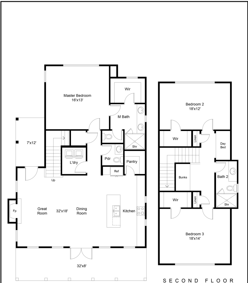
SECOND FLOOR
